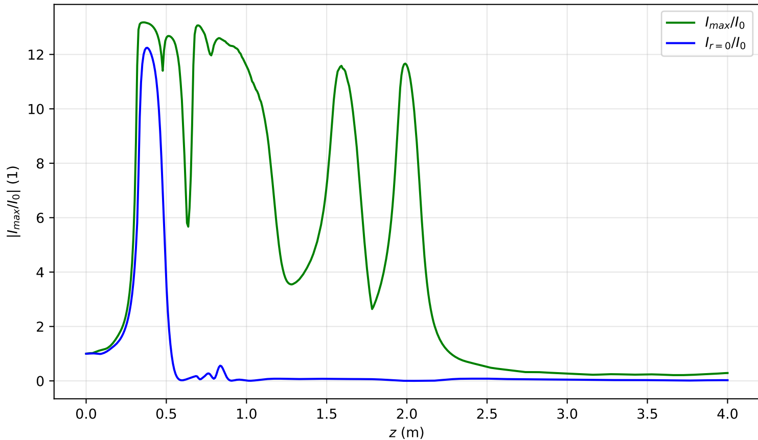
I_{max}(x=0, y=0, z)/I_0 , P_{in}=8.4P_{cr} , noisy input, artificial time
